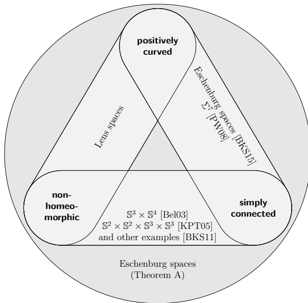
FIGURE 1. Existing results on pairs of distinct souls
