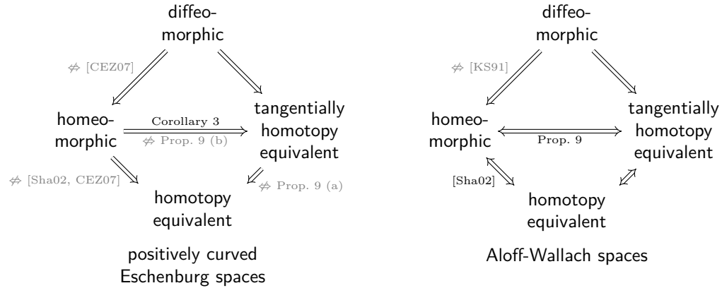
FIGURE 2. Implications between different notions of isomorphism for positively curved Eschenburg spaces and for the subfamily of Aloff-Wallach spaces, respectively. All indicated implications ( \Rightarrow ) are strict. The references in gray refer to counterexamples to the inverse implications.
